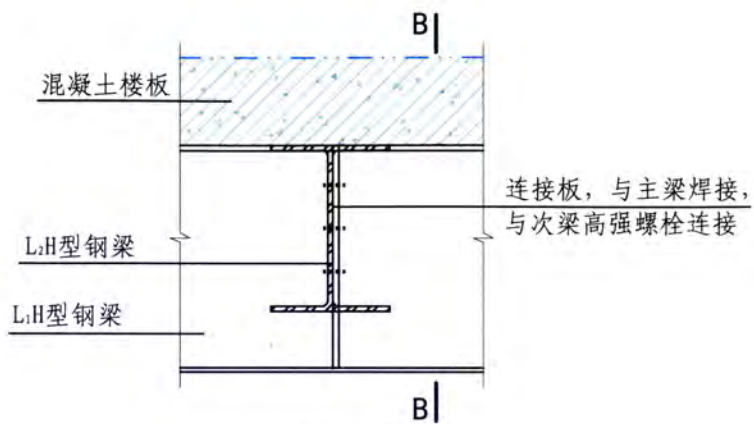
4-4
