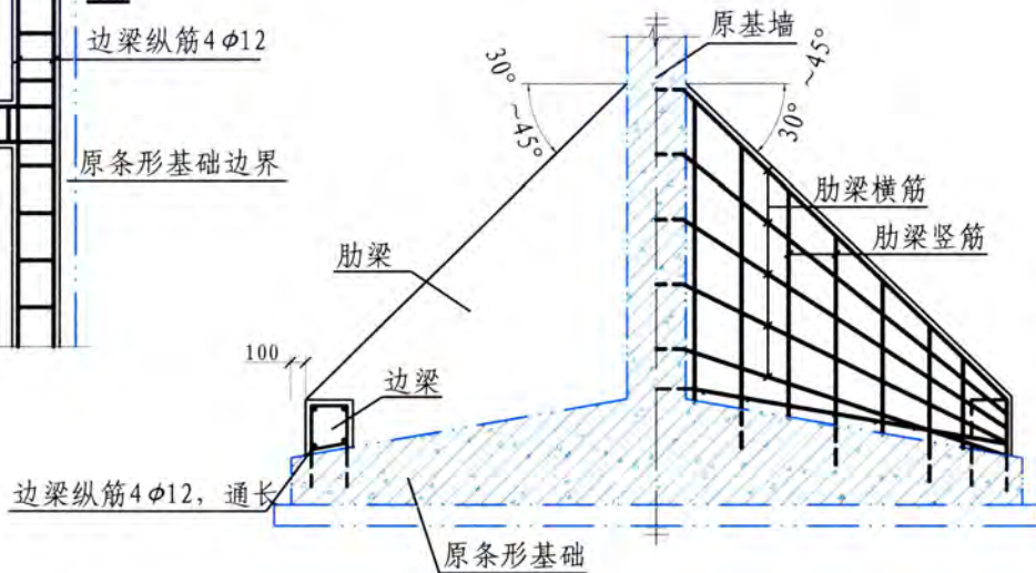
2-2
