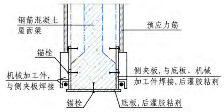
5-5
