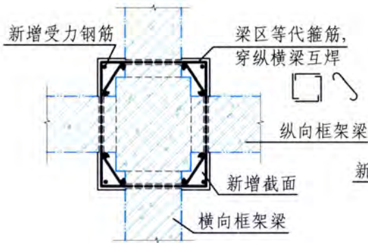
4-4
