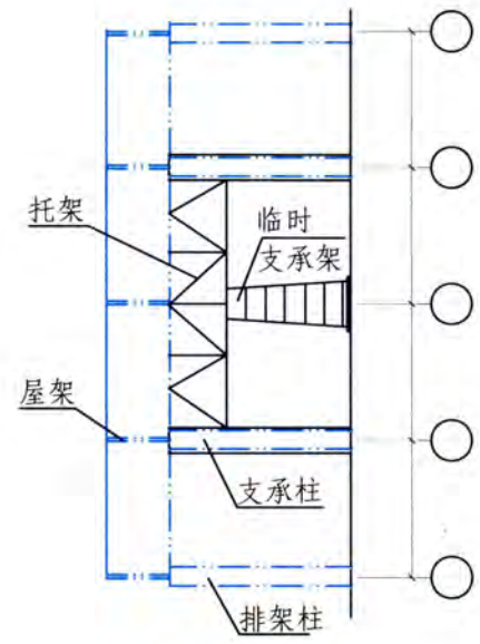
2-2
