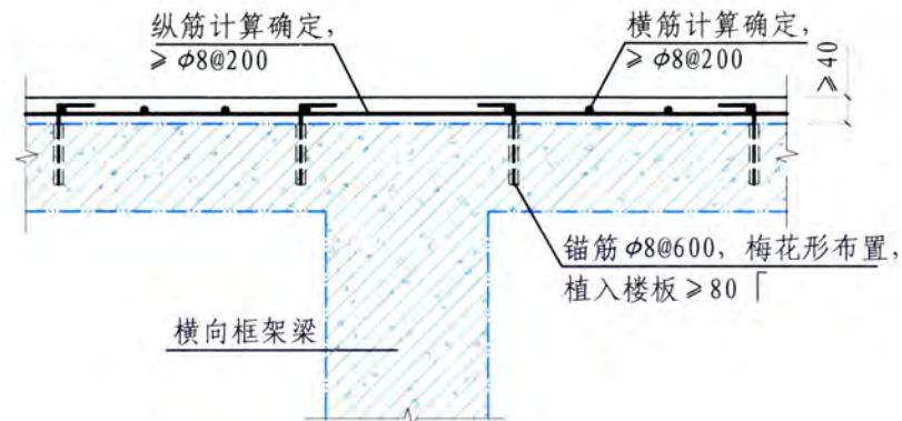
2-2
