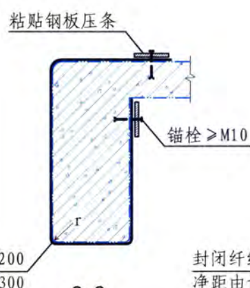
2-2 (钢板锚U形箍)
