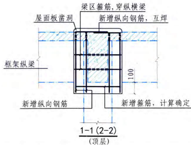
1-1 (2-2) (中间层)
