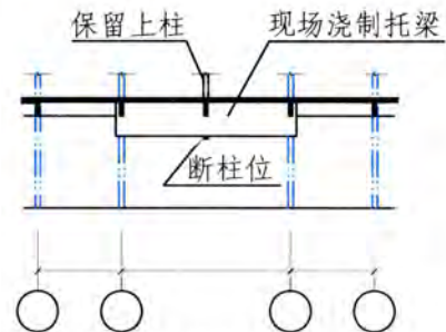
2-2 (断柱后)
