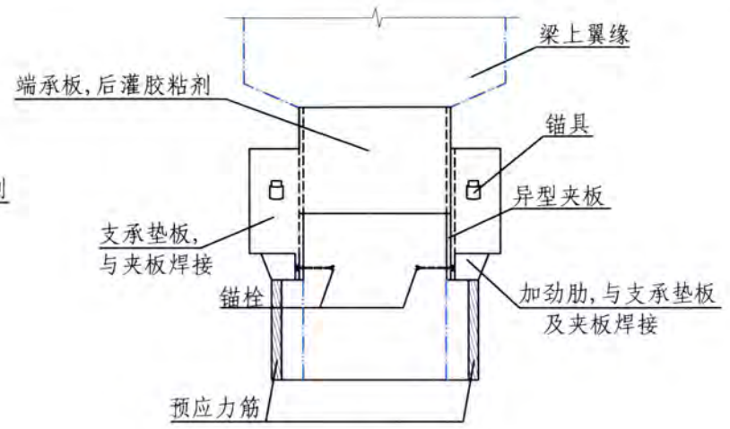
4-4
