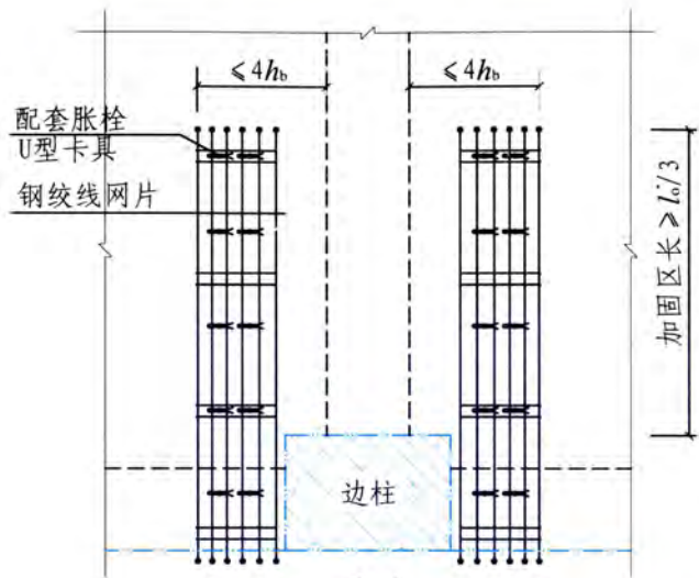
2-2 (边跨节点)
