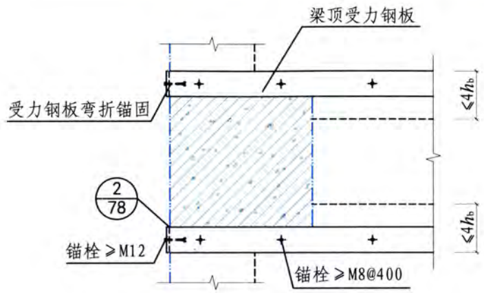
2-2 (梁顶有柱无墙时,弯折锚固)
