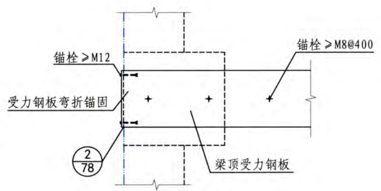
2-2 (梁顶无障碍时,弯折锚固)
